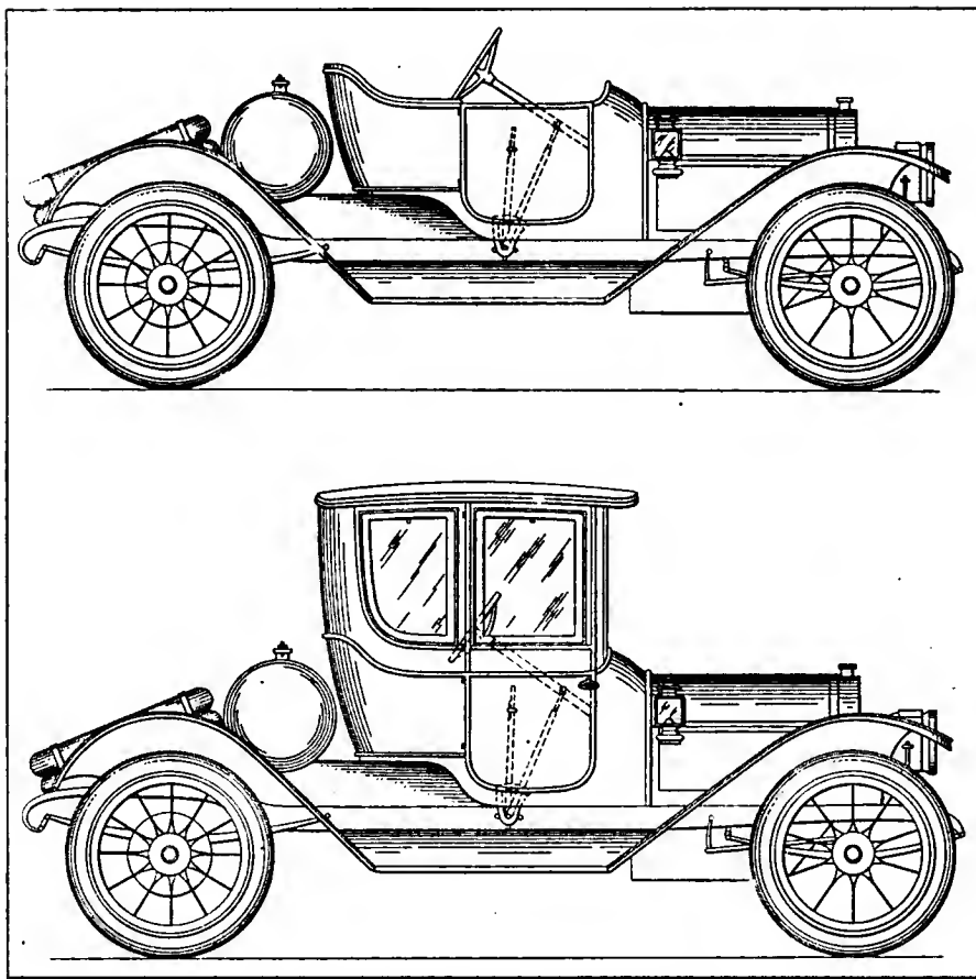
Fig. 4—Ordinary type of fore-door runabout for warm-weather use Fig. 5—Same car after upper part has been added to convert it into a coupé
